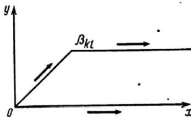
Pic.1. Contour [0, \beta_{k,l}] in complex plane \mathbb{C} .
